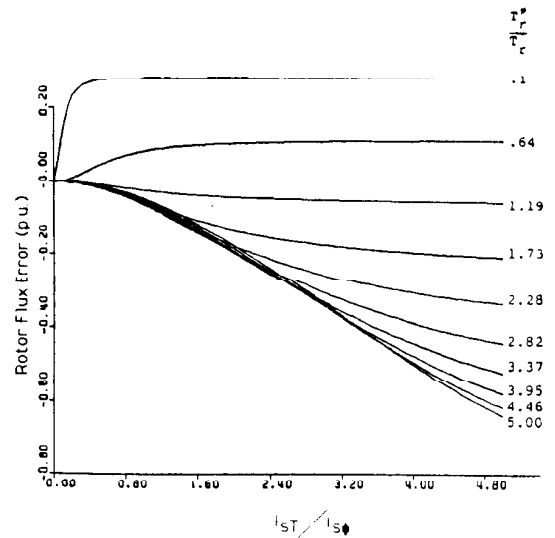
Fig. 6. Calculated flux transient for different input current ratios.
