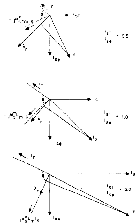
Fig. 7. Phasor diagrams showing rotor flux linkage for different current ratios with \tau_r^* = 0.1\tau_r .
