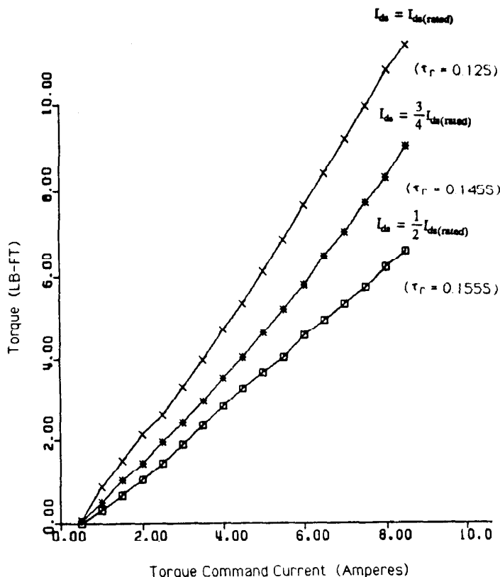
Fig. 17. Measured input-output torque curves for three different flux levels using 3-hp machine.
