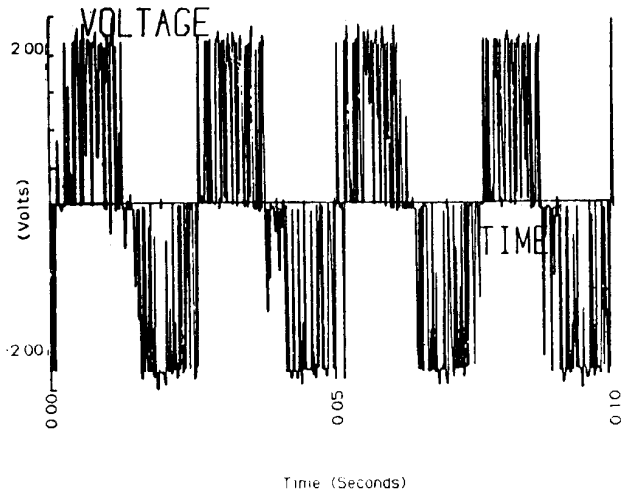
Fig. 8. Typical voltage waveform with sine-triangle-type CRPWM inverter.
