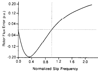
Fig. 5. Calculated flux error versus commanded slip frequency for 3-hp machine using proposed time constant test.
