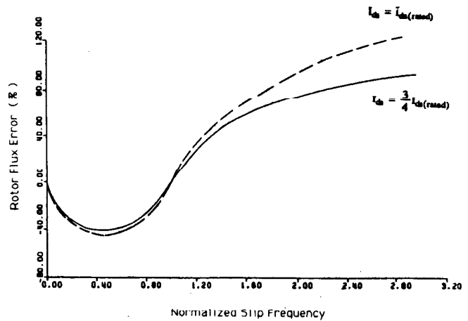
Fig. 16. Measured voltage transient versus slip frequency for different flux levels for 3-hp machine.
