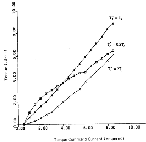
Fig. 13. Output torque versus steady-state torque command.
