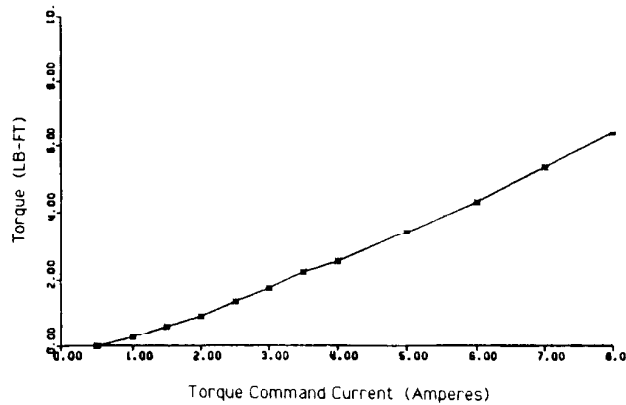
Fig. 15. Input-output torque relation for high-efficiency induction machine when controller is properly tuned by automated measurement system.
