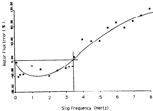
Fig. 12. Voltage error versus commanded slip frequency (3-hp machine) as measured by automated procedure.
