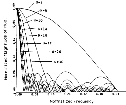
Fig. 10. Frequency response of moving average filter with increasing values of N .
