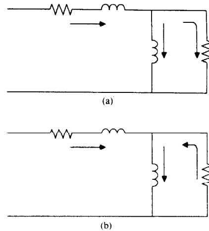
Fig. 4. Directions of motor currents during rotor time constant test. (a) Command frequency too large. (b) Command frequency too small.
