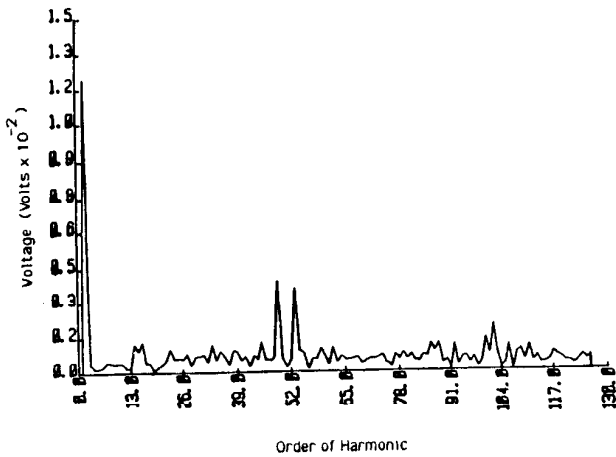
Fig. 9. Spectrum of voltage waveform in Fig. 7.
