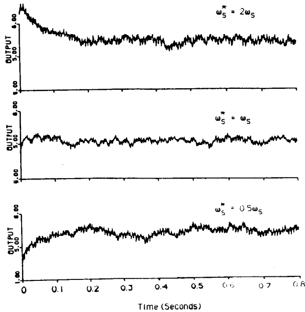
Fig. 11. Stator terminal voltage response for three different command frequencies.
