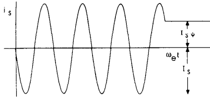
Fig. 3. Stator current test signal for rotor time constant measurement.
