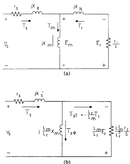
Fig. 2. (a) Conventional induction motor equivalent circuit. (b) Modified equivalent circuit.
