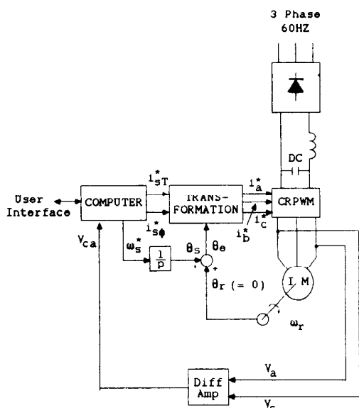
Fig. 1. Automated tuning system for rotor time constant measurement.
