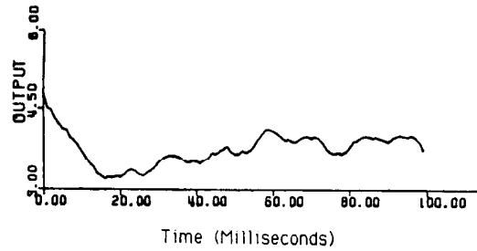
Fig. 14. Voltage transient for 1/3-hp machine when estimated rotor time constant is too small ( \tau_r^* = 0.5\tau_r ).
