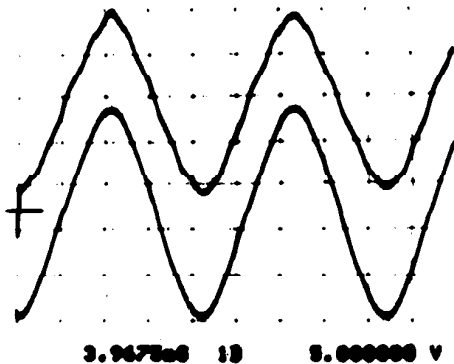
Fig. 4 Induced Voltage in Search Coil #01 (Upper Trace) and in Stator Phase c. Conditions: Stator Open Circuited, Rated Speed, Field Current I_{fd} = 1.45 Amperes.
