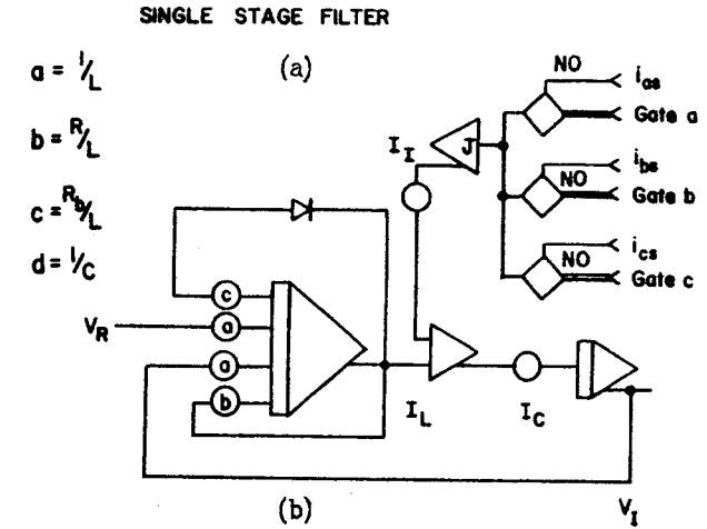
Fig. 5 (a) Equivalent Circuit of Single Stage Filter, (b) Analog Computer Simulation.
