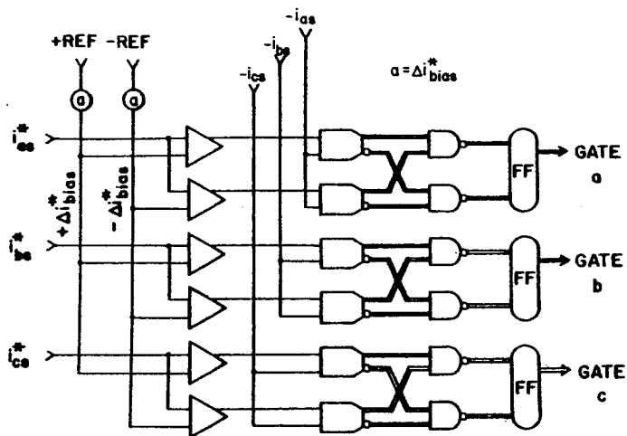
Fig. 7 Analog Computer Simulation of Hysteresis Type Gate Pulse Generator for PWM Inverter.
