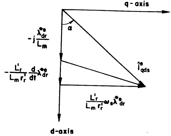
Fig. 2 Vector Diagram of Stator Current and Rotor Flux Linkage in the Synchronously Rotating Reference Frame.
