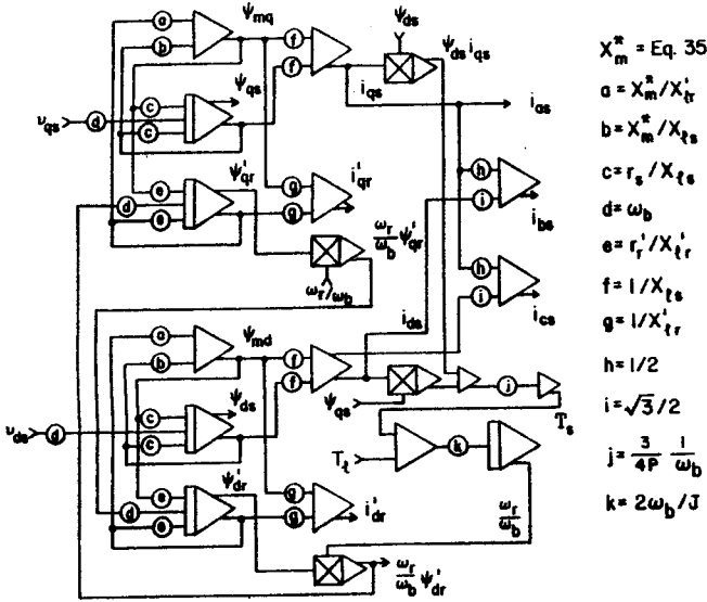
Fig. 4 A d, q Axes Simulation Diagram for an Induction Motor in the Stationary Reference Frame.
