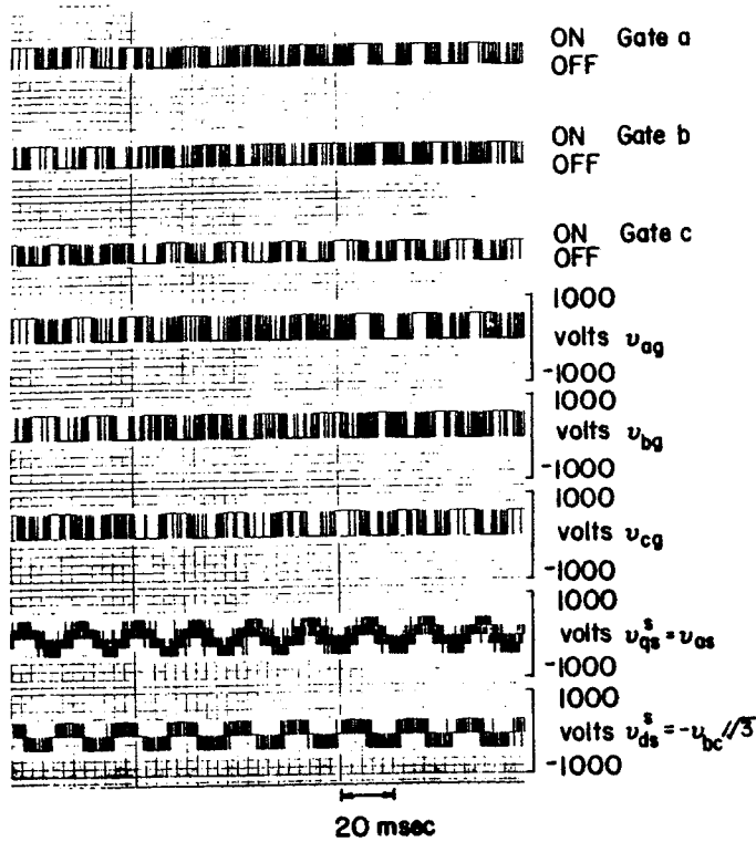
Fig. 12 Simulation Traces of Inverter Gate Pulses and Inverter Voltages.
