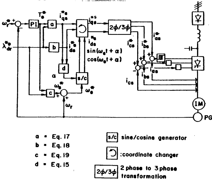
Fig. 3 Configuration for Indirect Field Oriented Control.
