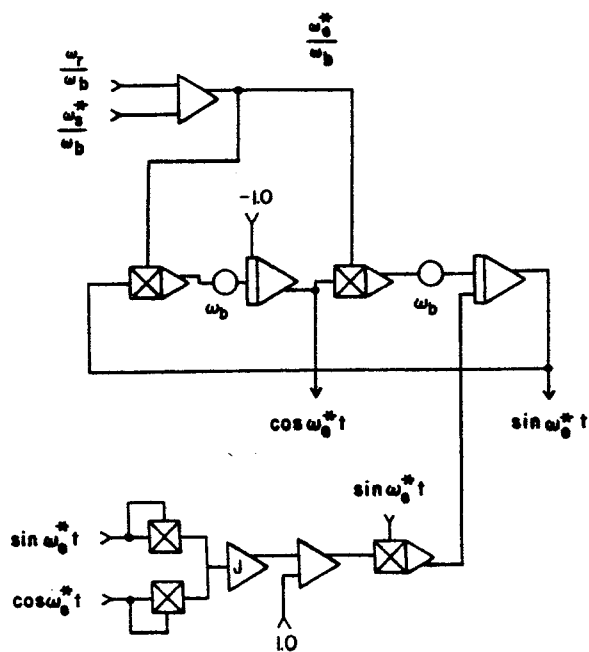
Fig. 9 Simulation Diagram Showing Mechanization of Variable Frequency Generator for Reference Frame Transformation.
