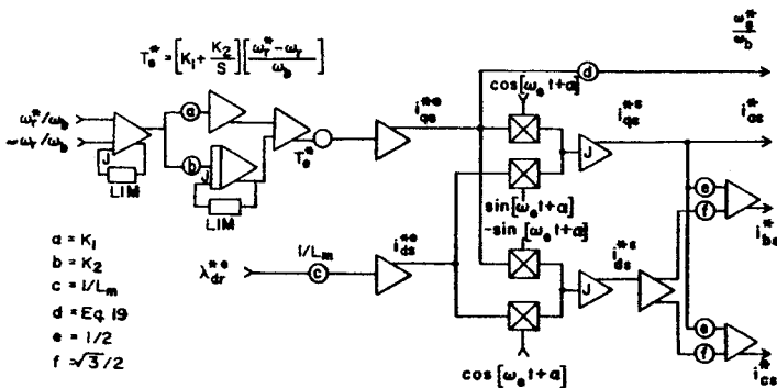
Fig. 8 Simulation Diagram for Field Oriented Controller Showing Independent Regulation of Flux and Torque and Transformation from Rotating to Stationary Axes.
