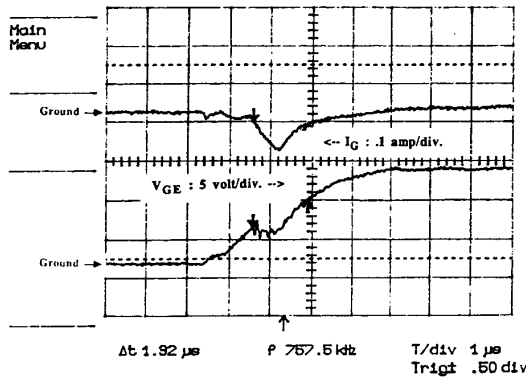
Fig. 4 Turn-On Gating Characteristics of IGBT.
