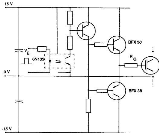
Fig. 3 IGBT Drive Circuit.
