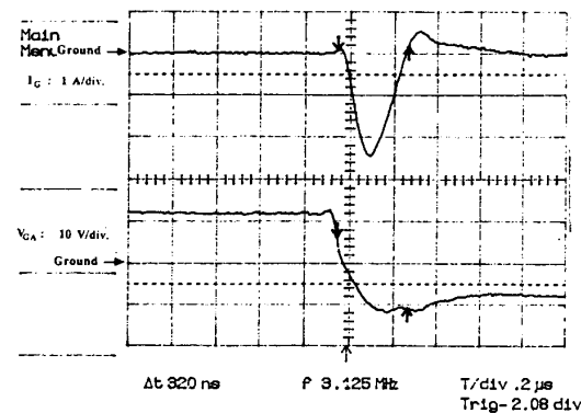
Fig. 7 Gating Characteristics of MCT at Turn-On.
