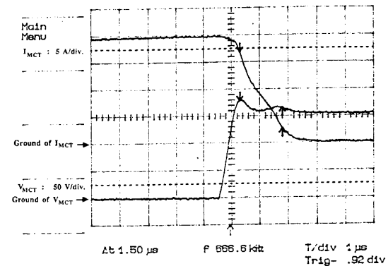
Fig. 12 Detailed View of Chopper Circuit of Fig. 10 Showing Turn-Off of MCT.
