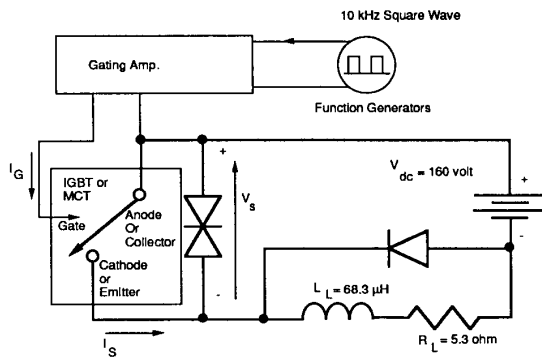
Fig.9: Chopper Circuit Used for the Device Test.
