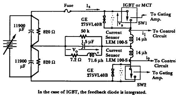
Fig. 15 Parallel Output Series Resonant (POSR) Converter Configuration Used for the Test.
