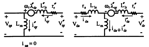
Fig. 6: Equivalent Circuit for Mode II.
