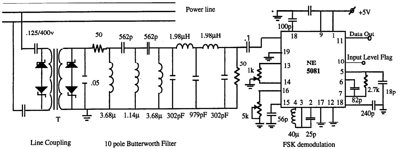
Fig 5 Prototype Receiver Circuit
