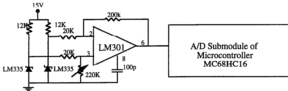
Fig 6 Data Acquisition Circuit for Winding Temperature Measurement
