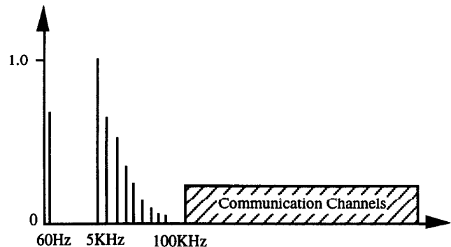
Fig. 2 Transmission Characteristics of a Typical PWM Inverter-Fed Power Line
