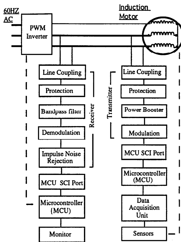
Fig. 3 Schematic of the New Motor Condition Monitoring System
