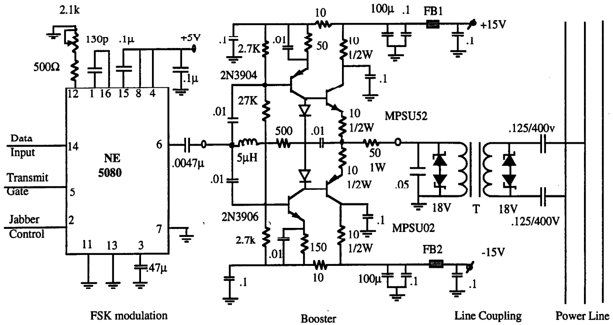
Fig. 4 Prototype Transmitter Circuit
