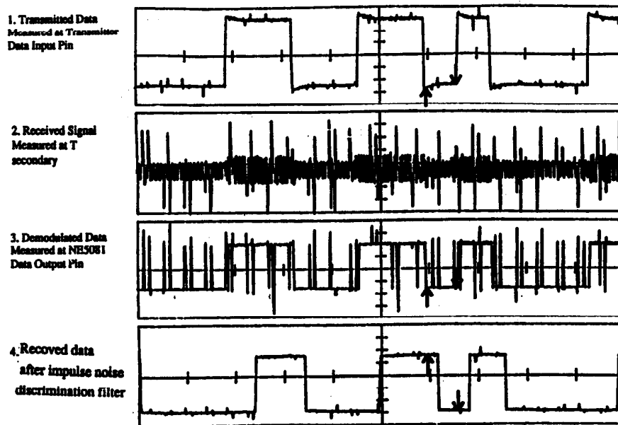
Fig. 8 Receiver Waveforms with a Data Baud Rate of 9600 bps
