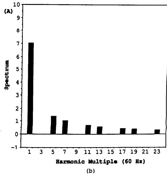
Fig.4: (a) Input phase voltage and input line current of phase control in which shift angle \phi is lagging, (b) Harmonics content of input line current i_{ain} shown in (a).
