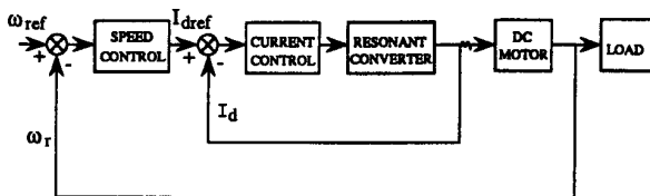
Fig.8 Block diagram of the control system.
