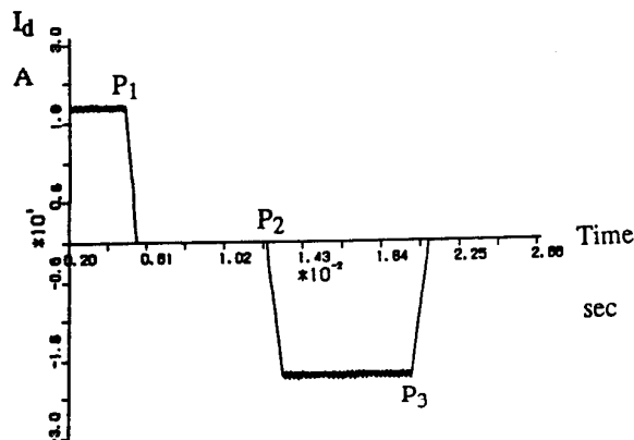
Fig.10 Response of I_d when current reference is changed stepwisely.
