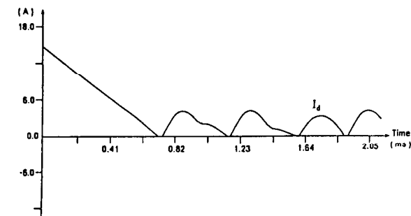
Fig.7 Motor current I_d when I_d^* steps to zero at t=0 .
