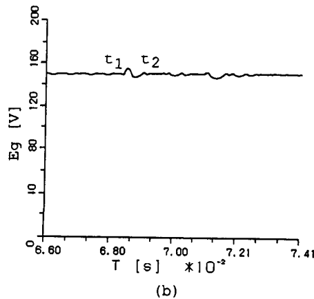
Fig.6 Motor speed response of resonant converter method, (a) when E_g reference is changed from 150 V to 100 V, (b) when the load R_L is changed from 20\Omega to 40\Omega .
