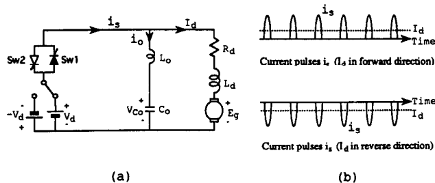
Fig.9 The monophase circuit of SRDCL Dual Converter and Resonant current pulses i_s .
