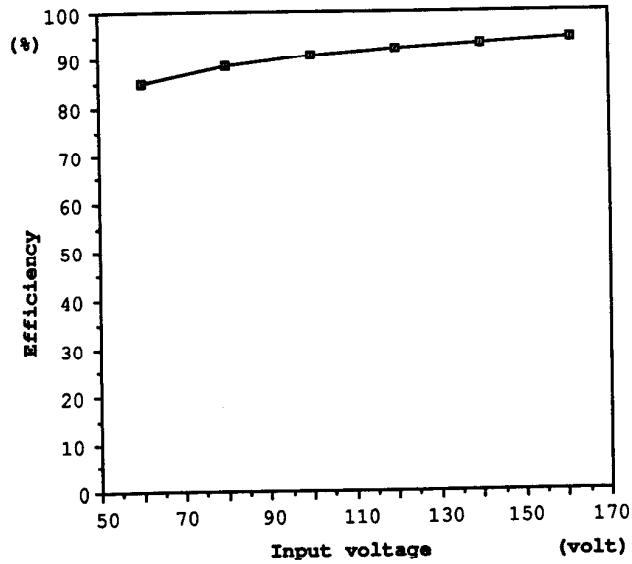
Fig.14 Efficiency of the experimental model
