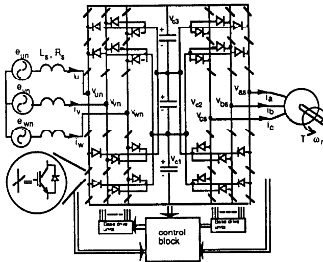
Fig. 8 Simulated four level rectifier inverter drive system
