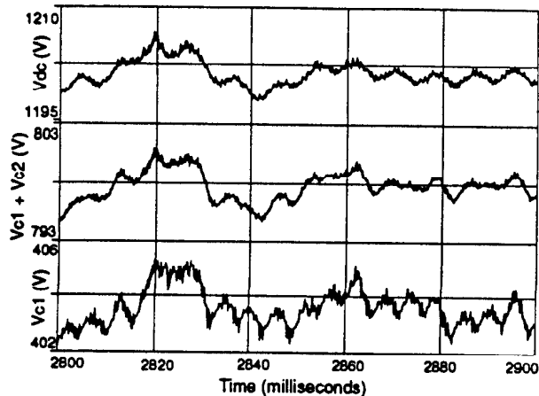
Fig. 11 DC bus voltages (unsaturated inverter)
