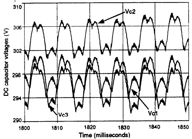
Fig. 19 Capacitor voltages (saturated inverter)
