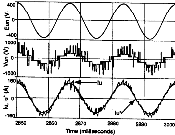
Fig. 10 Rectifier unity power factor operation (unsat. inverter)
