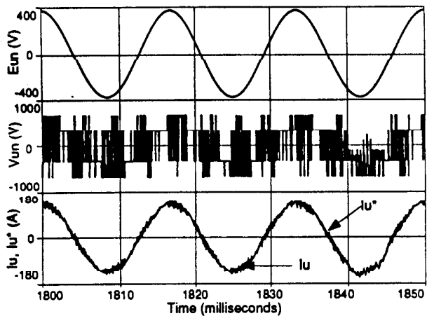
Fig. 16 Rectifier unity power factor operation (saturated inverter)
