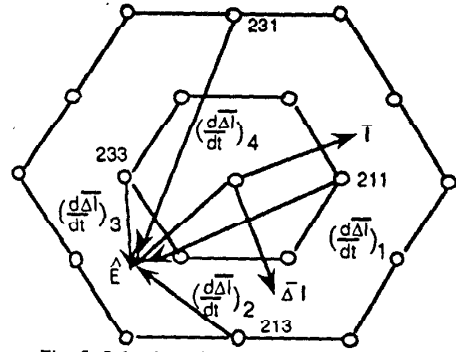
Fig. 5 Selection of rectifier switching states
