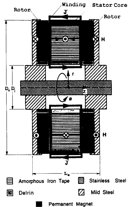
Fig. 1 AFTPM Machines
