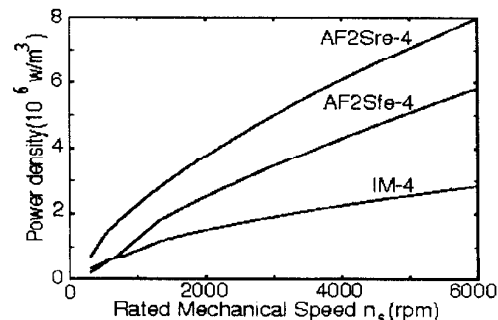
Fig. 6 Power densities comparison between induction machines and AF2SPM machines. ( A = 60,000 A/m , J_s = 6.2 \times 10^6 A/m^2 , P_R = 75,000 w .)
