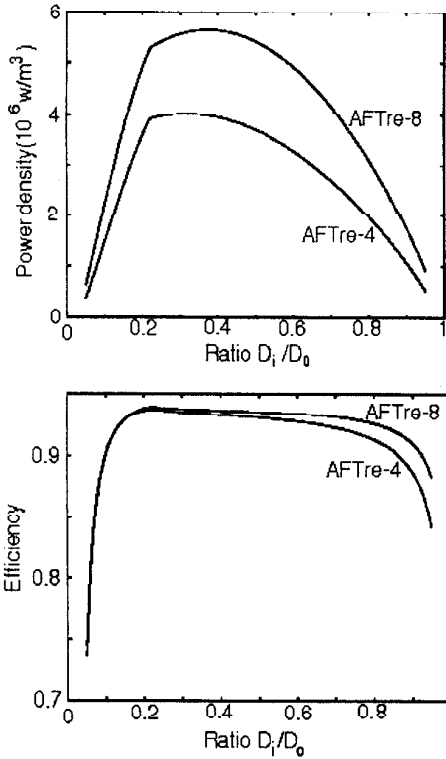
Fig. 2 Power density and efficiency of the AF2SPM machine vs. ratio \lambda . A = 60,000 \text{ A/m} , J_s = 6.2 \times 10^6 \text{ A/m}^2 , P_n = 75,000 \text{ w} , n_s = 3000 \text{ rpm} , p = 2 (AFTre-4), p = 4 (AFTre-8), using rare earth PM.
