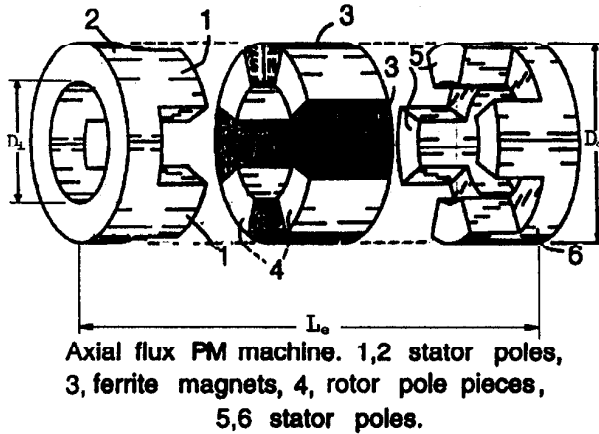
Fig. 3 AF2SPM Machines
