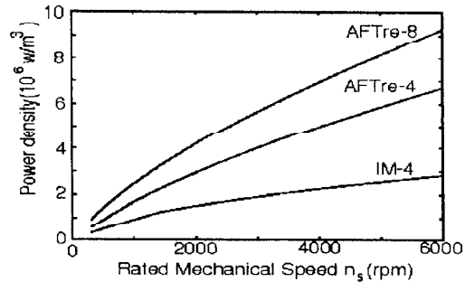
Fig. 5 Power densities comparison between induction machines and AFTPM machines ( A = 60,000 A/m , J_s = 6.2 \times 10^6 A/m^2 , P_R = 75,000 w ).
