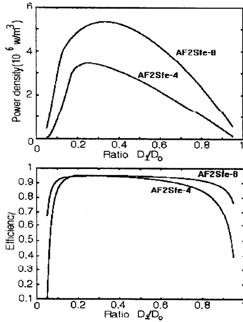
Fig. 4 Power density and efficiency of the AF2SPM machine vs. ratio \lambda . A = 60,000 A/m , J_s = 6.2 \times 10^6 A/m^2 , P_R = 75,000 w , n_s = 3000 rpm, p = 2 (AF2Sfe-4), p = 4 (AF2Sfe-8), using ferrite PM.
