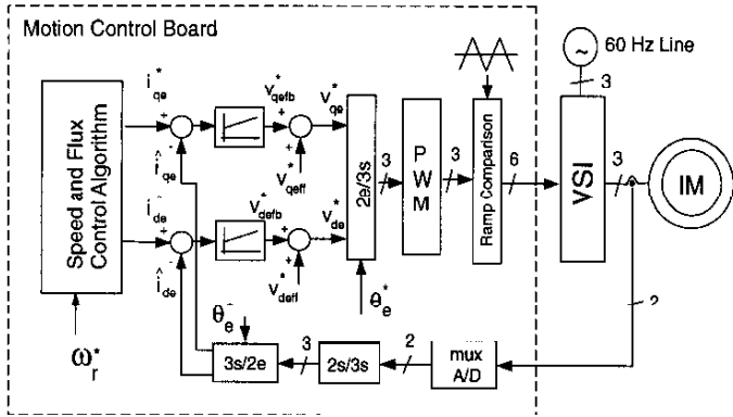
Fig. 6. High performance induction motor drive system diagram.
