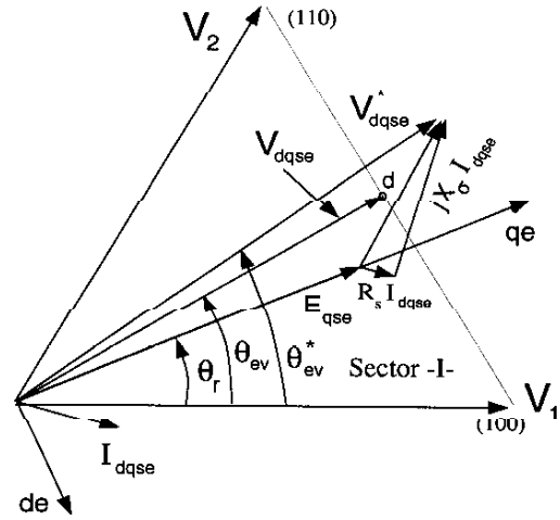
Fig. 14. Synchronous frame rotor flux oriented induction motor voltage vector diagram illustrated along with the inverter voltage vector diagram.
