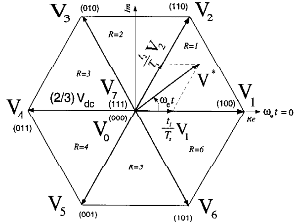
Fig. 4. The space vector diagram illustrates the direct digital implementation principle. The upper switch states are shown in the bracket as (Sa+, Sb+, Sc+) and "1" is "on" state while "0" corresponds to "off" state.
