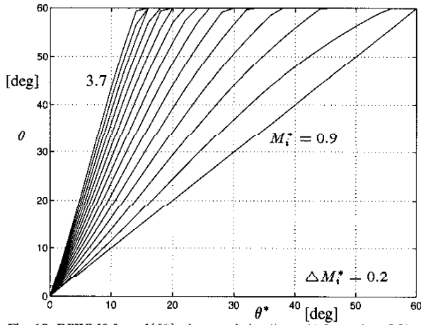
Fig. 10. DPWM0 \theta = f(\theta^*) characteristics ( \zeta_0 = 1 ) for various M_i^* values. M_i^* starts at 0.9 and increments with 0.2 units.
