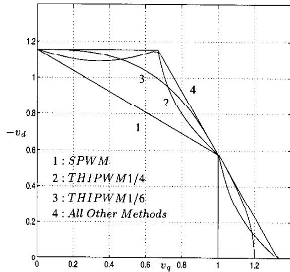
Fig. 19. Vector space illustration of the modulator per carrier cycle voltage linearity limits. All voltage vectors are normalized to \frac{V_{dc}}{2} .
