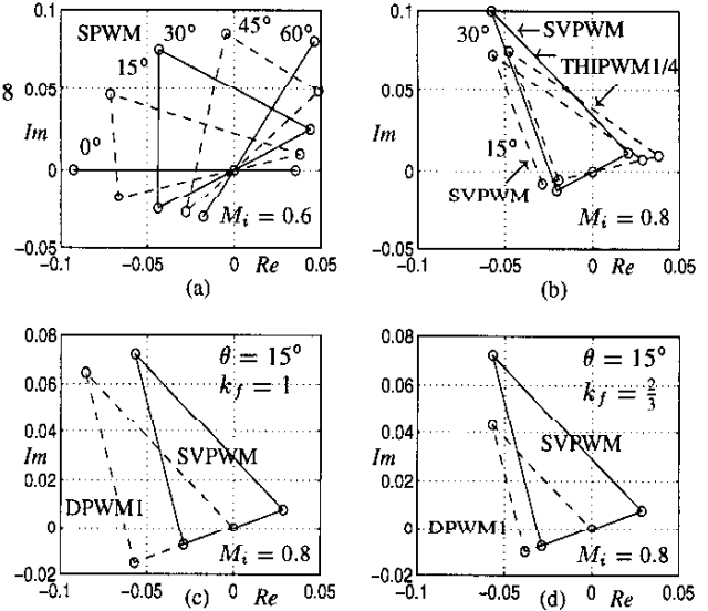
Fig. 10. The switching frequency harmonic flux trajectories of various PWM methods. (a): SPWM, (b): SVPWM and THIPWM1/4 compared for \omega_e t = 15^\circ and \omega_e t = 30^\circ values, (c): SVPWM and DPWM1 compared for k_f = 1 , (d): SVPWM and DPWM1 for k_f = \frac{2}{3} .
