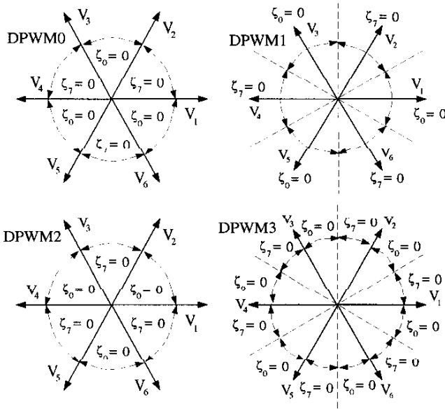
SVPWM: \zeta_0 = \zeta_7 = 0.5 DPWMMAX: \zeta_0 \rightarrow 0 DPWMMIN: \zeta_7 = 0
