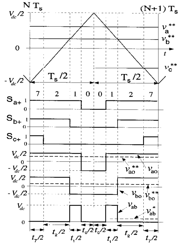
Fig. 5. The per carrier cycle view of switch logic signals, inverter states, and VSI output voltages for 0 \leq w_e t \leq \frac{\pi}{3} ( R = 1 ).
