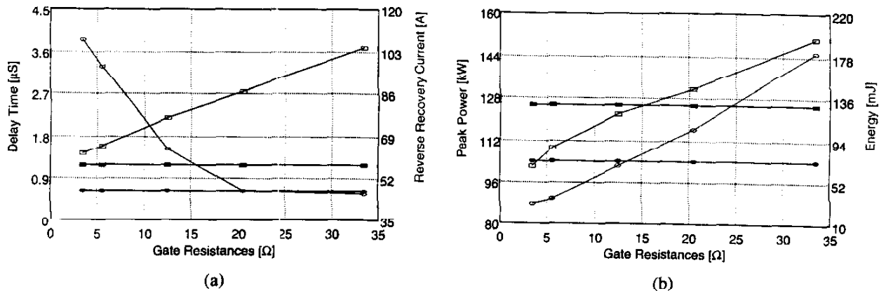
Fig. 8. Comparison of turn-on characteristics between the AGD and the CGD as gate resistance is varied. (a) Investigation of the turn-on delay time, T_{d(CGD)} and T_{d(AGD)} , and the peak reverse recovery current, I_{rr(CGD)} and I_{rr(AGD)} . (b) Investigation of the peak power, P_{on(CGD)} and P_{on(AGD)} , and the turn-on energy loss, E_{on(CGD)} and E_{on(AGD)} . Operating conditions are as follows: V_{dc} = 600V , I_L = 350A , V_{gs+} = 18V , V_{gs-} = -12V .
