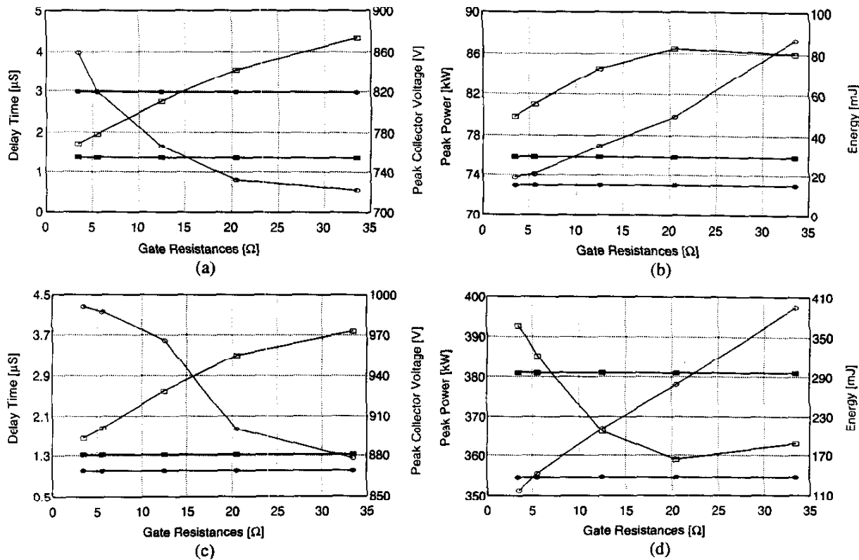
Fig. 12. Comparison of turn-off characteristics between the AGD and the CGD as the gate resistance is varied. I_L = 150A in charts (a) and (b). I_L = 620A in charts (c) and (d). (a) and (c) investigate the delay time, T_d(CGD) and T_d(AGD) , and the peak collector voltage, V_{ce(CGD)} and V_{ce(AGD)} . (b) and (d) investigate the peak power, P_{off(CGD)} and P_{off(AGD)} , and the energy loss, E_{off(CGD)} and E_{off(AGD)} . Operating conditions are as follows: V_{dc} = 600V , V_{gg+} = 18V , and V_{gg-} = -12V .
