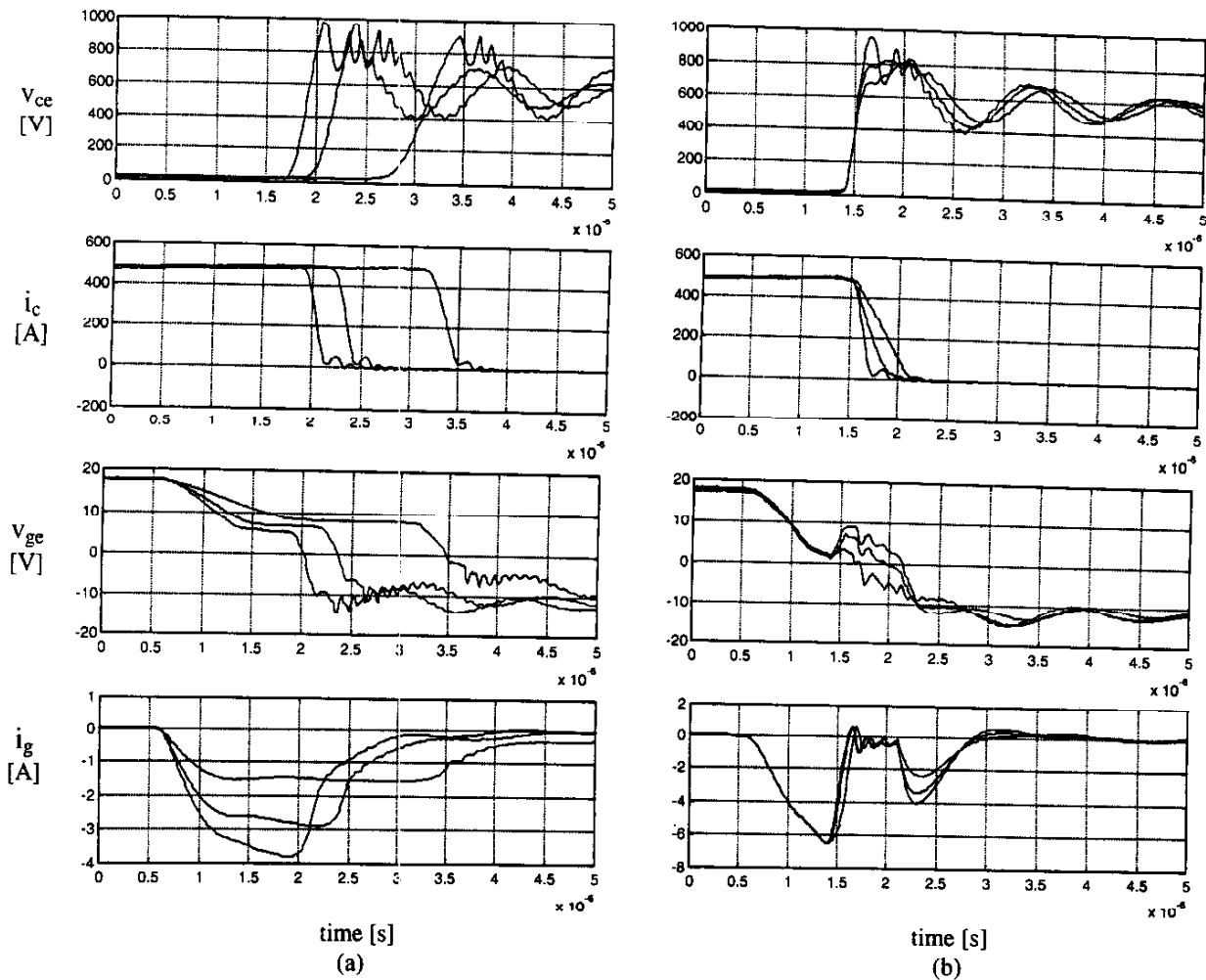
Fig. 10. Measured turn-off switching waveforms ( v_{cc} , i_c , v_{ge} , i_g ) with (a) the CGD and (b) the AGD when the turn-off di/dt is varied. Turn-off gate resistors used in the CGD for varying di/dt are 3.5, 5.6, 12.5 \Omega . Other conditions are as follows: V_{dc} = 600V , I_L = 500A , V_{gg+} = 18V , V_{gg-} = -12V .
