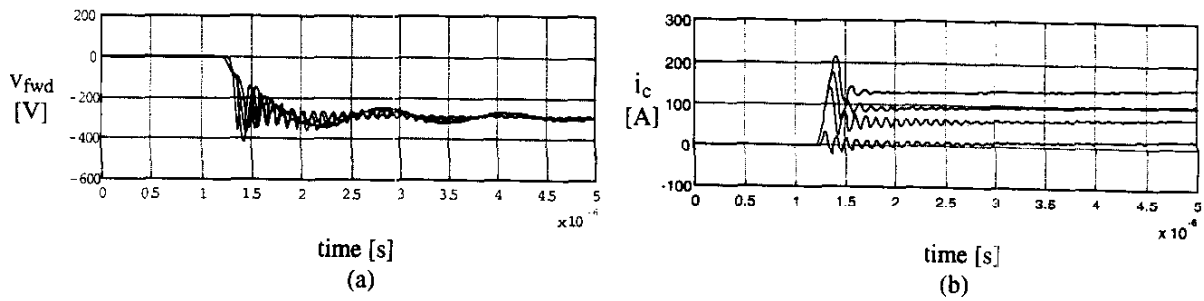
Fig. 6. Measured turn-on waveforms with the CGD at current levels of 0, 50, 80, 120A when the gate resistor of 0.5\Omega is used. (a) The free-wheeling diode voltage. (b) The collector current. Other conditions are as follows: V_{dc} = 300V , V_{eg+} = 18V , V_{eg-} = -12V .
