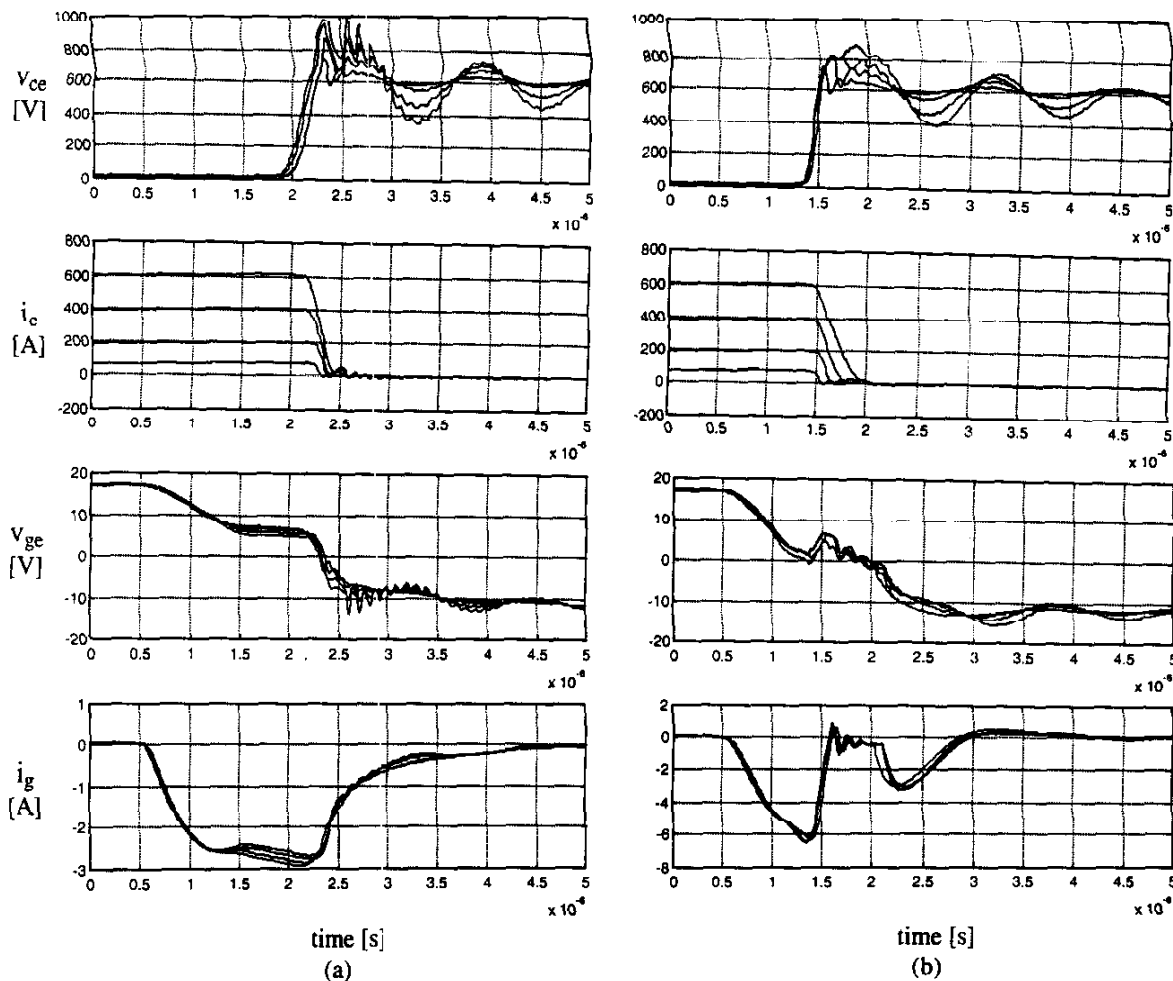
Fig. 9. Measured turn-off switching waveforms ( v_{ce} , i_c , v_{ge} , i_g ) with (a) the CGD and (b) the AGD at current levels of 80, 205, 405, 620A. Turn-off gate resistor used in the CGD is 5.6\Omega . Other conditions are as follows: V_{dc} = 600V , V_{gg+} = 18V , V_{gg-} = -12V .
