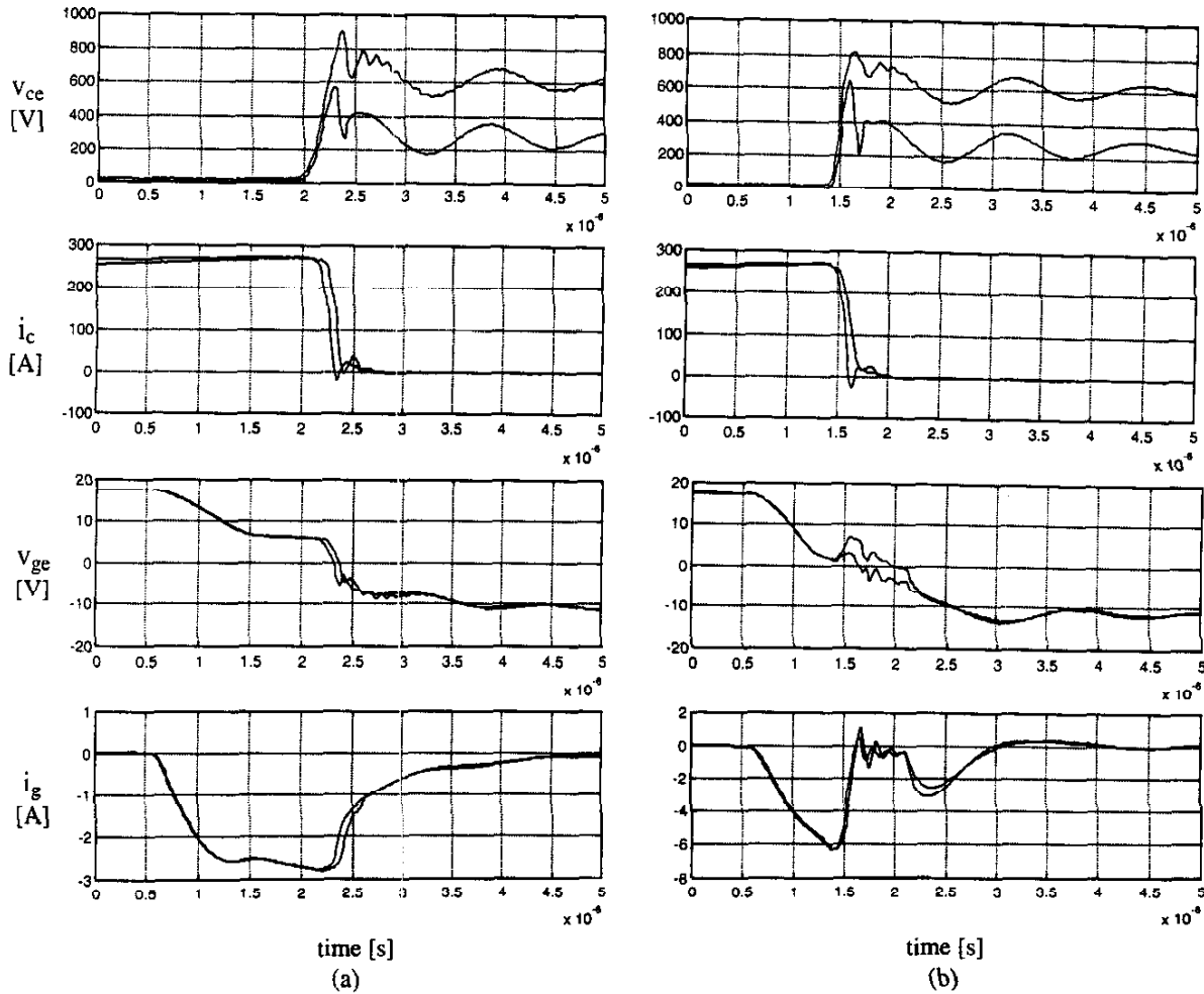
Fig. 11. Measured turn-off switching waveforms ( v_{ce} , i_c , v_{ge} , i_g ) with (a) the CGD and (b) the AGD when the dc bus voltage is varied. The dc bus voltages are 300, 600V. Turn-off gate resistor used in the CGD is 5.6\Omega . Other conditions are as follows: I_L = 270A , V_{gs+} = 18V , V_{gs-} = -12V .
