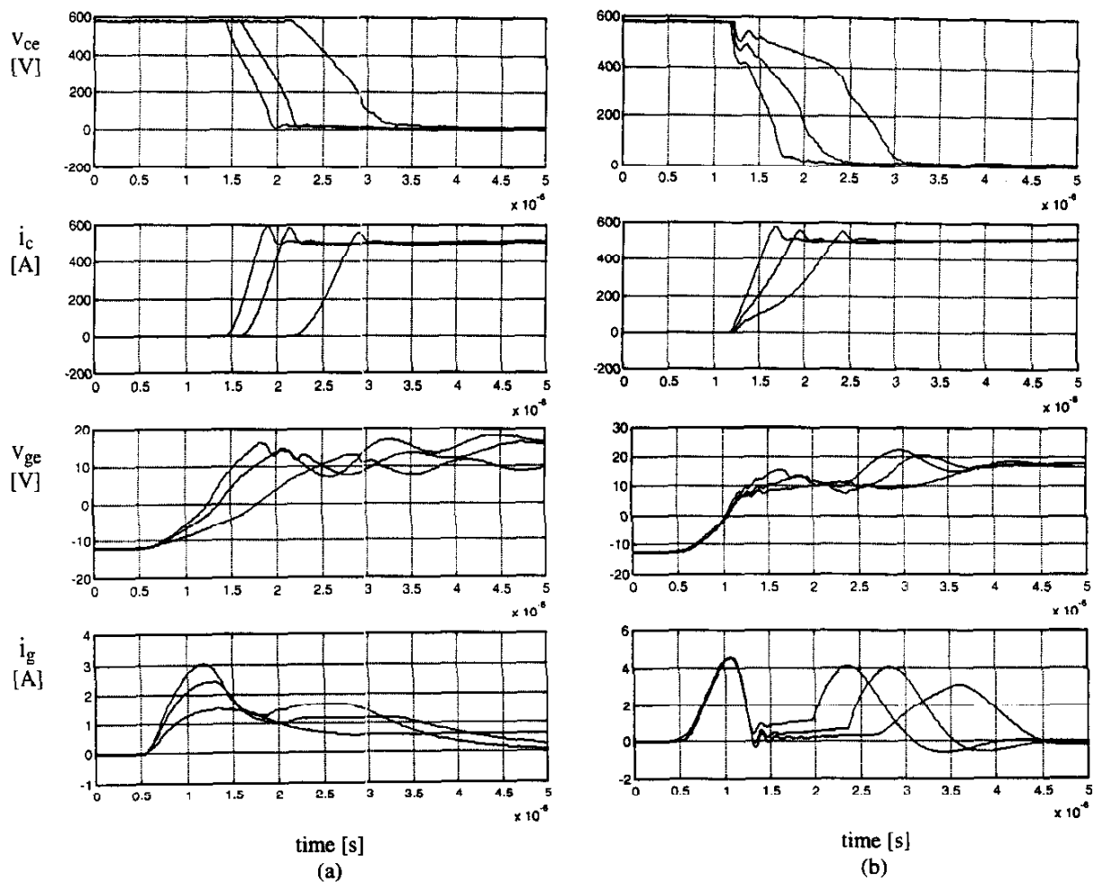
Fig. 7. Measured turn-on switching waveforms ( V_{ce} , i_c , V_{ge} , i_g ) with (a) the CGD and (b) the AGD when the turn-on di/dt is varied. Turn-on gate resistors used for varying di/dt in the CGD are 3.5, 5.6, 12.5Ω. Other conditions are as follows: V_{dc} = 600V , V_{eg+} = 18V , V_{eg-} = -12V .
