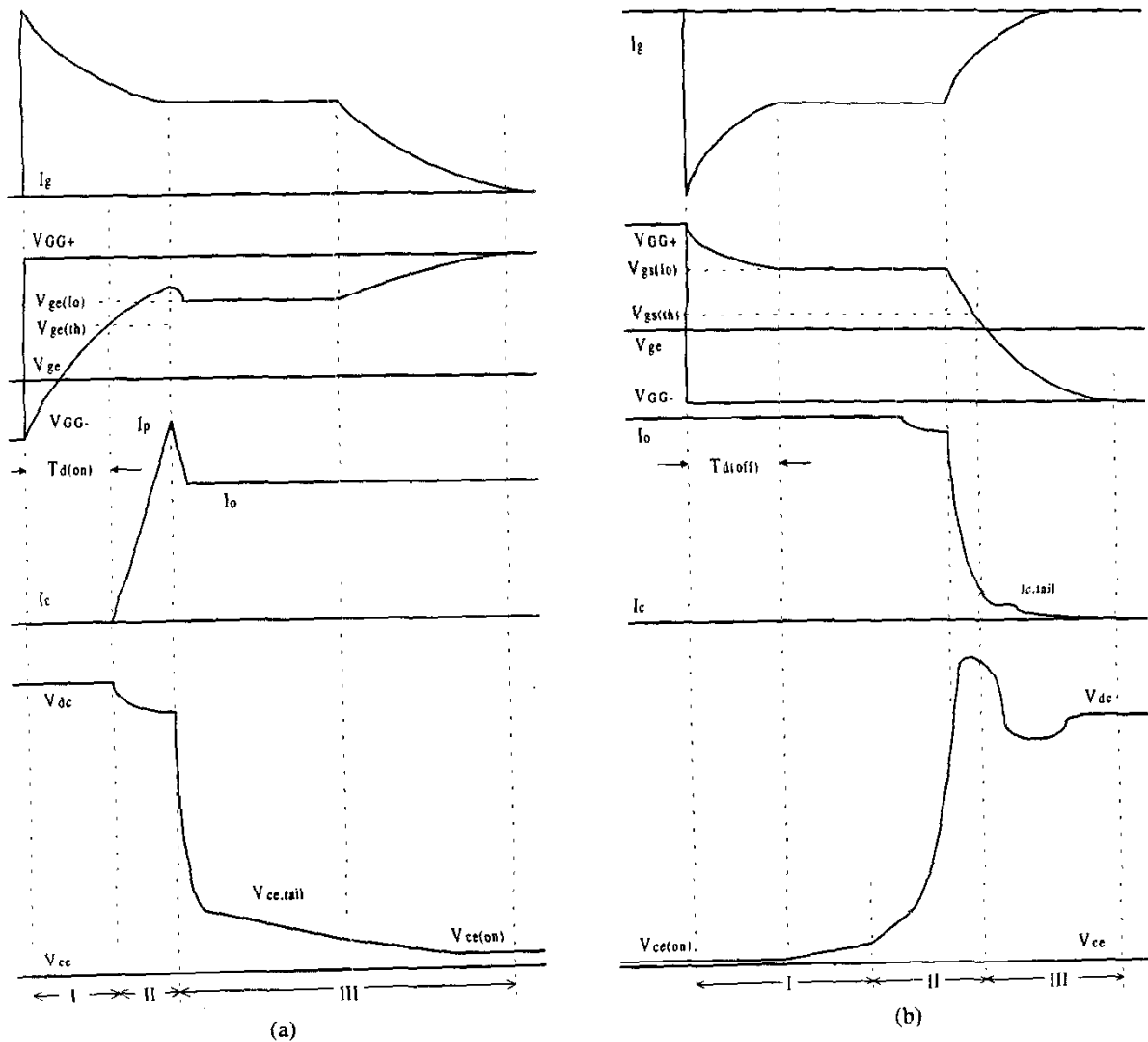
Fig. 1. Sketches of (a) turn-on and (b) turn-off waveforms of an IGBT under inductive load switching with a CGD circuit.
