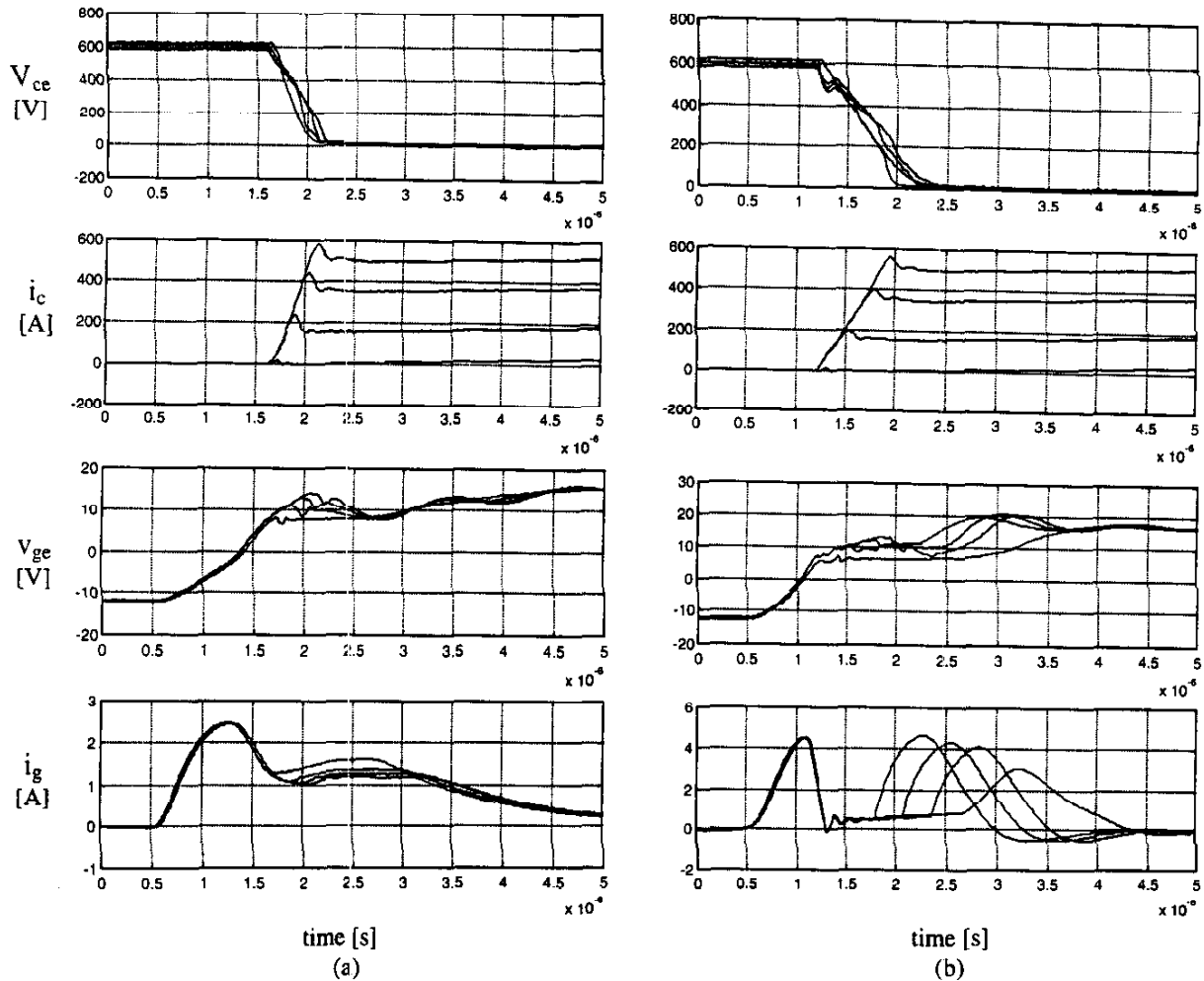
Fig. 5. Measured turn-on switching waveforms ( v_{ce} , i_c , v_{ge} , i_g ) with (a) the CGD and (b) the AGD at current levels of 0, 150, 350, 500A. Turn-on resistor of 5.6\Omega is used in the CGD. Other conditions are as follows: V_{dc} = 600V , V_{gg+} = 18V , V_{gg-} = -12V .
