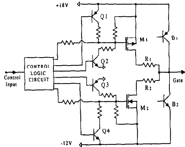
Fig. 4. Schematic of the proposed AGD circuit.
