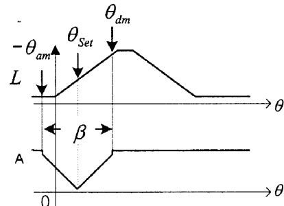
Fig. 4 Determination of set angle & optimal \beta for the proposed encoder
