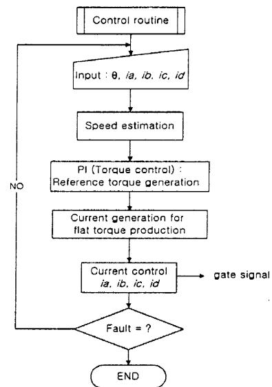
Fig. 7 Control routine
