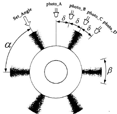
Fig. 2 Proposed linear encoder
