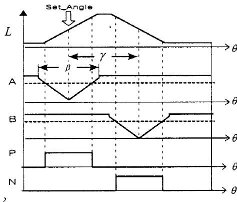
Fig. 3 Switching patterns
