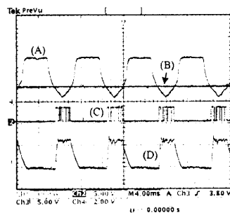
Fig. 9 Experimental waveforms of control signal and phase current corresponding output of photo-Tr. with the peak current control method (A) output of photo-Tr. (B) reference signal (B) (C) control signal (D) corresponding phase current
