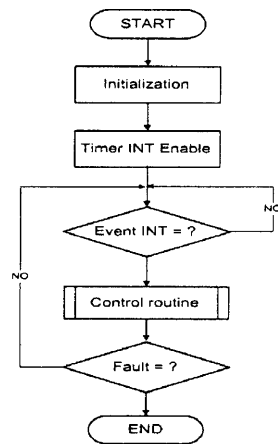
Fig. 6 Flowchart of main routine
