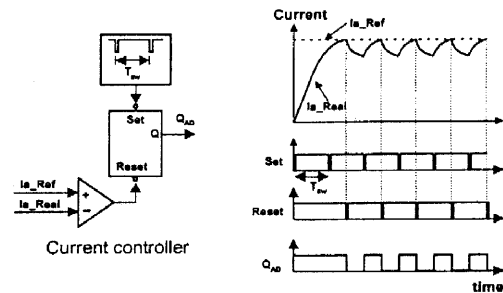
Fig. 5 Current controller & Key waveforms
