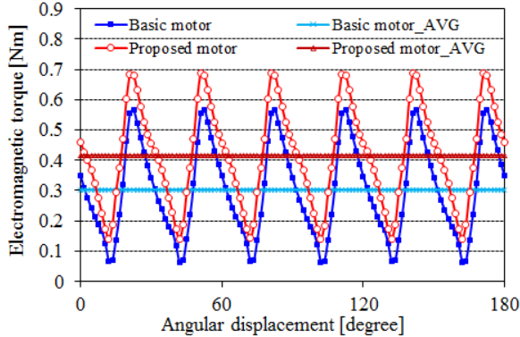
Fig. 6. Electromagnetic torque of the basic and proposed motors.
