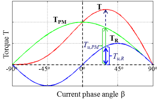
Fig. 2. Typical torque characteristics. T : resultant torque, T_{PM} : magnetic torque, T_R : Reluctance torque.
