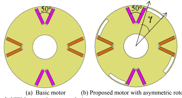
Fig. 3. VIPM motors in concept design.
