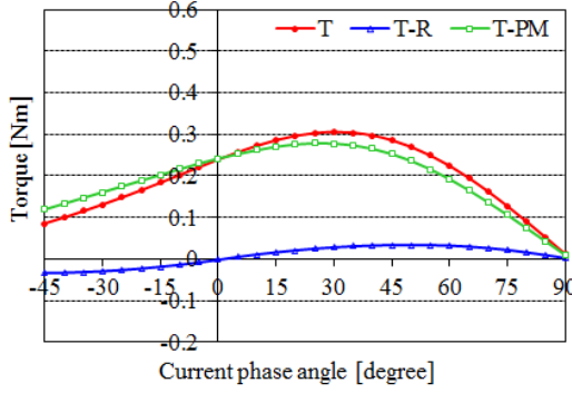
(a) Basic motor
