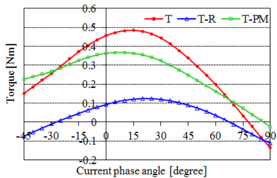
Fig. 9. Torque characteristics of the optimized motor. T: resultant torque, T_{PM} : magnetic torque, T_R : Reluctance torque.
