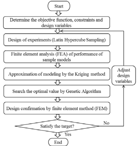
Fig. 7. Optimal design process.
