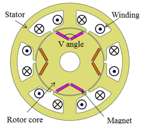
Fig. 1. Configuration of the conventional V-type IPM motor.
