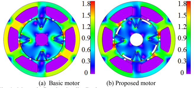
Fig. 4. Magnetic flux density distribution.
