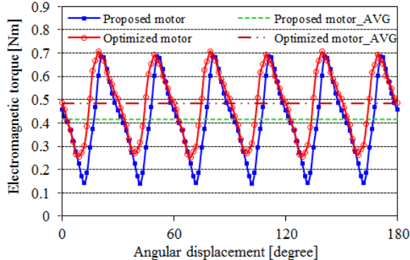
Fig. 10. Comparison of electromagnetic torque.
